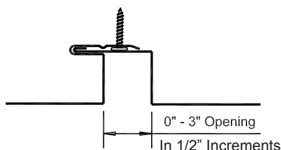
Seam to Lock Detail
